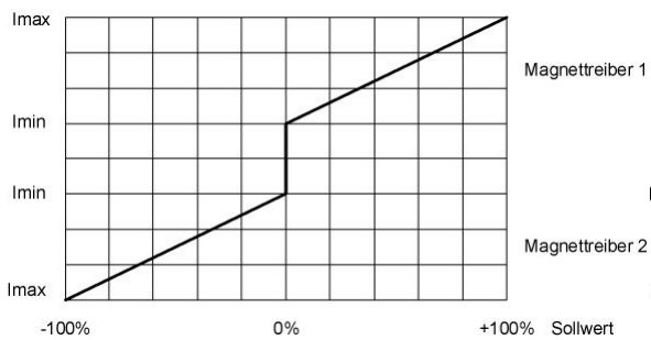
Standard 2-Magnet
